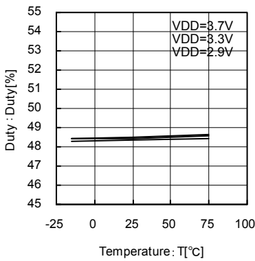
Fig.62 54MHz Temperature - Duty
