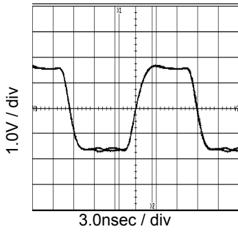
Fig.44 54MHz output waveform VDD=3.3V, at CL=15pF
