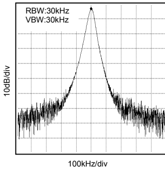
Fig.40 Spectrum Waveform (VDD=3.3V, Select="L", Output=50MHz)
