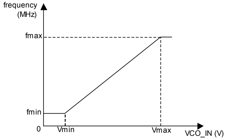
Fig.60 VCO Characteristics
