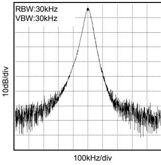
Fig.37 Spectrum Waveform (VDD=3.0V, Select="L", Output=50MHz)
