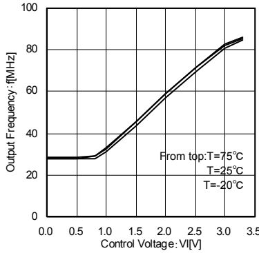
Fig.32 Control Voltage – Output Frequency (VDD=3.3V, Rbias=2.4KΩ)
