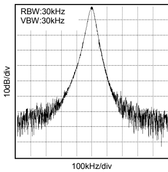
Fig.43 Spectrum Waveform (VDD=5.0V, Select="L", Output=75MHz)
