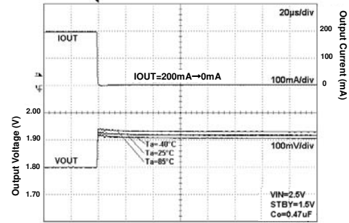
Fig 19. Load Response
