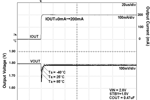
Fig 18. Load Response
