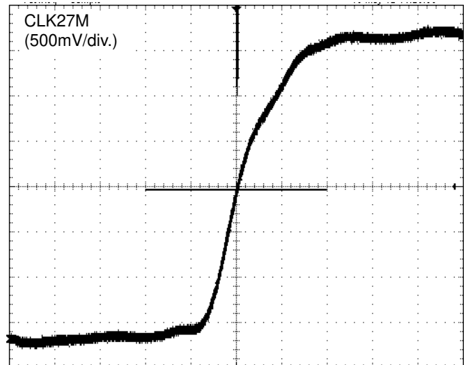
Figure 6. CLK27M Period-Jitter
