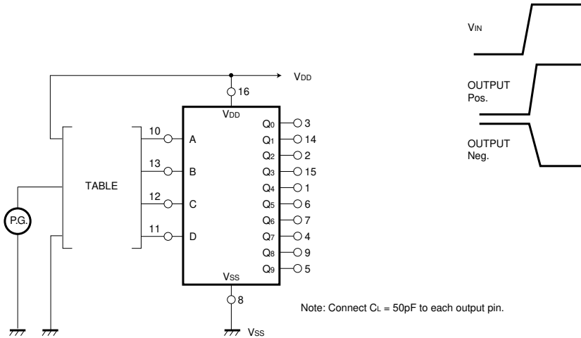
Fig. 2 Switching characteristics measurement circuit
