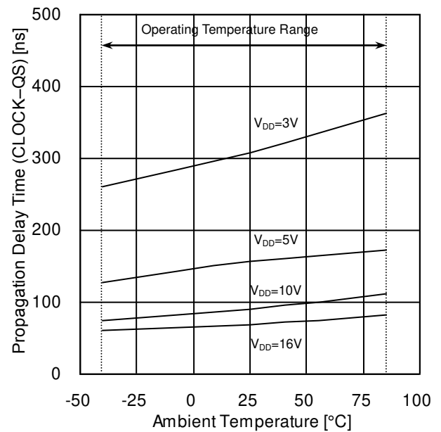
Figure 4. Propagation Delay Time t_{PHL} (CLOCK-QS) vs Ambient Temperature
