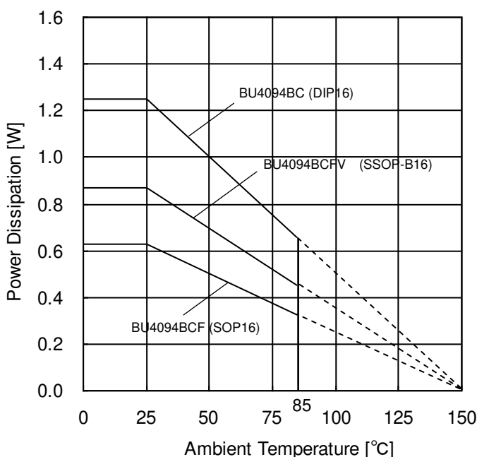
Figure 19. Derating Curve
