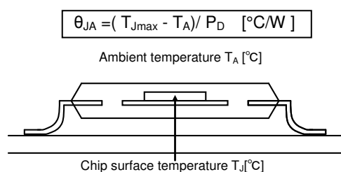
Figure 18. Thermal resistance
