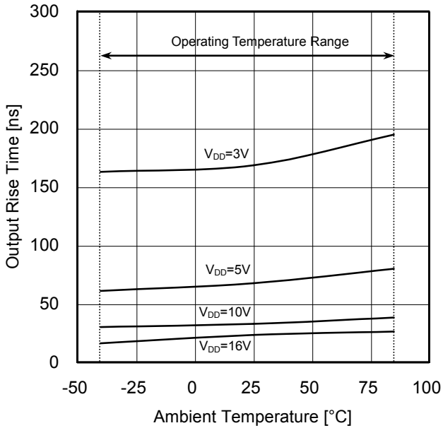
Figure 7. Output Rising Time t_{LH}
