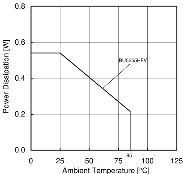
(c) BU5255HFV
