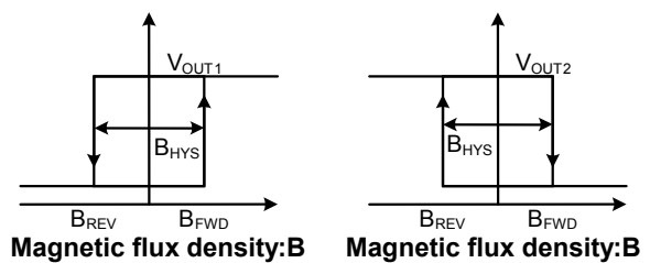
Figure 2. Output operation
