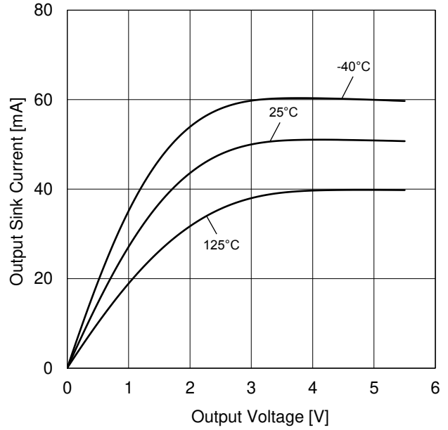
Figure 11. Output Sink Current vs Output Voltage (V DD =5.5 V)
