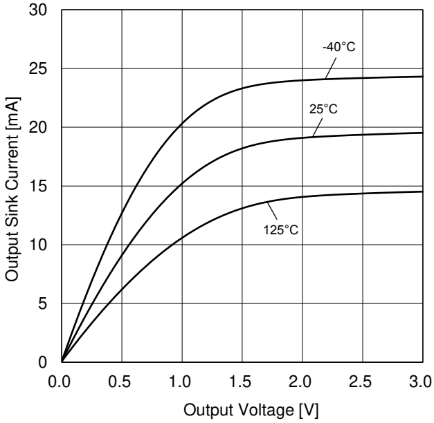
Figure 10. Output Sink Current vs Output Voltage (V DD =3 V)
