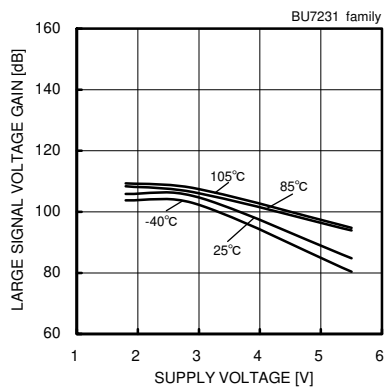
Fig. 60 Large Signal Voltage Gain – Supply Voltage
