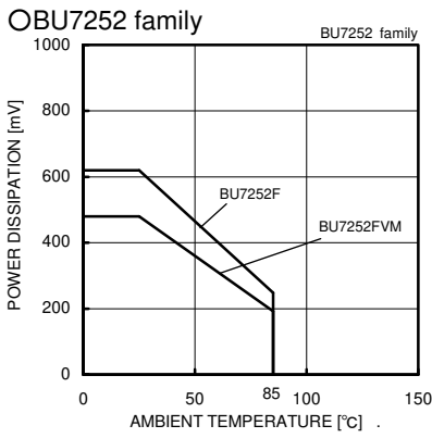
Fig. 23 Derating Curve
