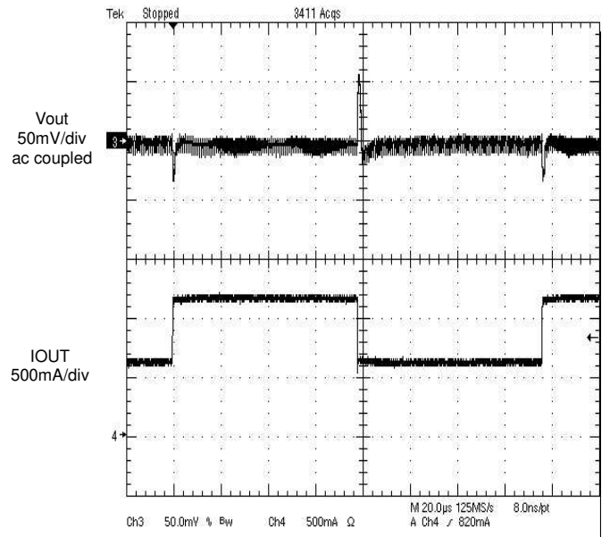
Figure 15. Load transient response 600mA to 1200mA t_r=t_f=100\text{ns} , MODE : Low
