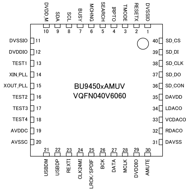
Figure 4. Arrangement of Terminals (BU9450xAMUV)
