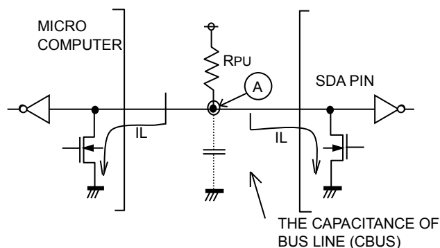
Figure 16. I/O Circuits
