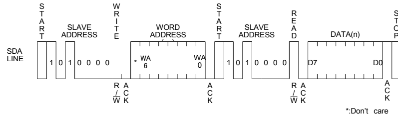
Figure 7. Random Read Cycle Timing
