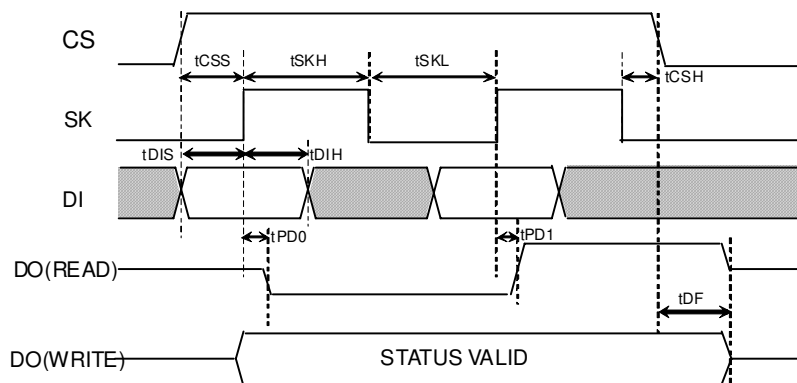
Figure 1. Sync data input / output timing
