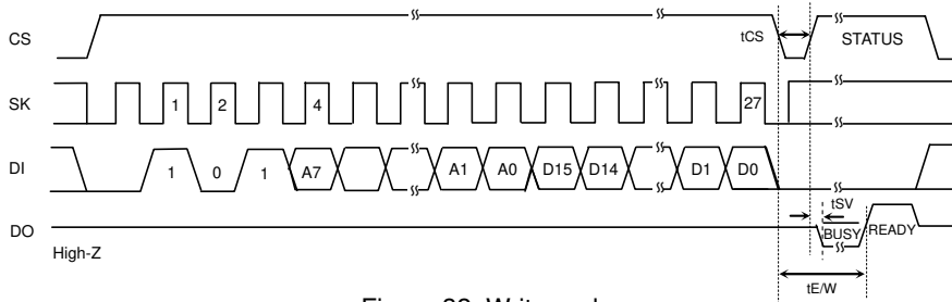
Figure 32. Write cycle
