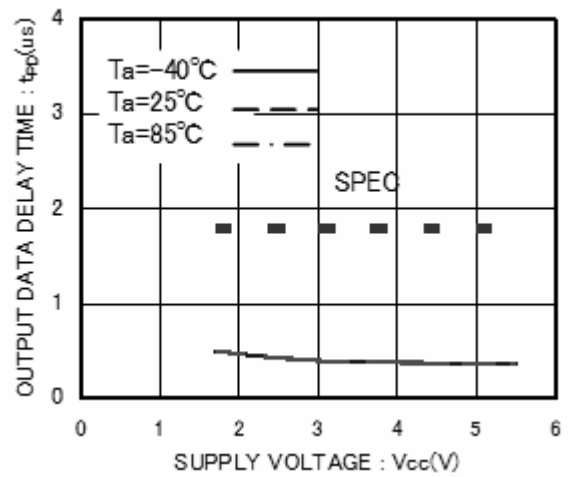
Figure 21. "H" Data output delay time t_{PD1}
