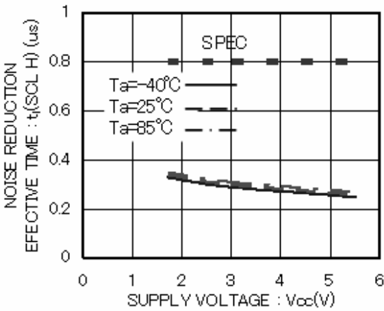
Figure 24. Noise reduction effective time t I (SCL H)
