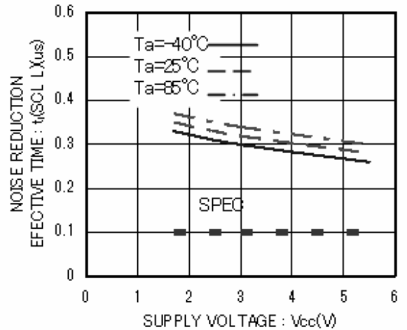
Figure 25. Noise reduction effective time t I (SCL L)
