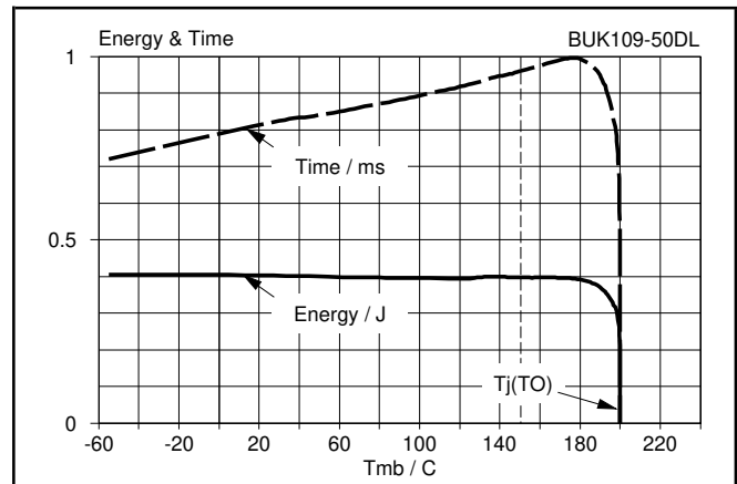
Fig. 11. Typical overload protection characteristics. Conditions: V_{DD} = 13\text{ V} ; V_{IS} = 5\text{ V} ; SC load = 30\text{ }\Omega
