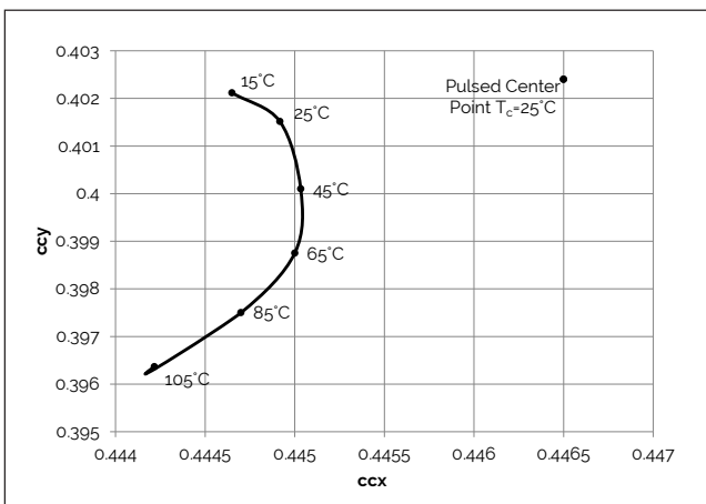
Figure 13: 3000K, 90 CRI Color Shift vs. Case Temperature 1,3
