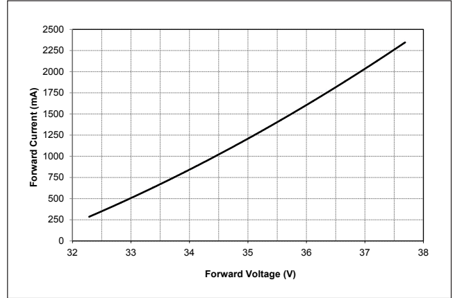
Figure 2: V18C Drive Current vs. Voltage
