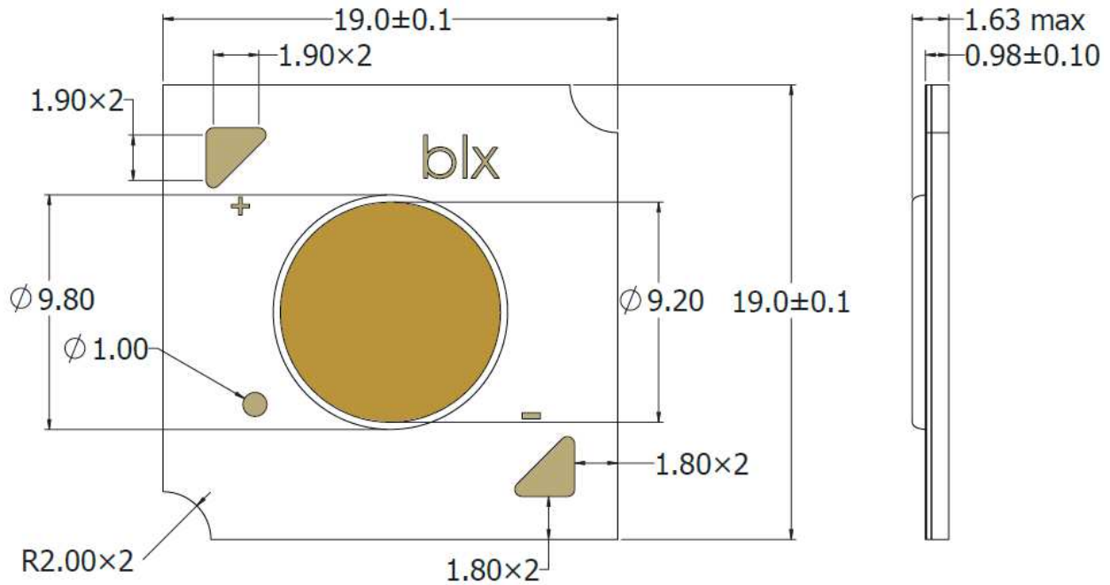
Figure 14: Drawing for Vg HD LED Array
