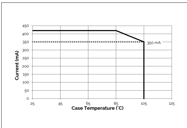
Figure 14: Derating Curve 6W, 12W
