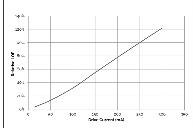
Figure 8: 4W Relative LOP vs. Drive Current, T_c=25^\circ\text{C}
