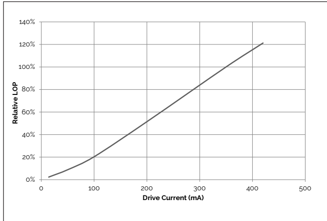
Figure 9: 6W Relative LOP vs. Drive Current, T_c=25^\circ\text{C}
