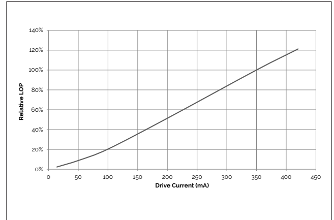
Figure 10: 12W Relative LOP vs. Drive Current, T_c=25^\circ\text{C}
