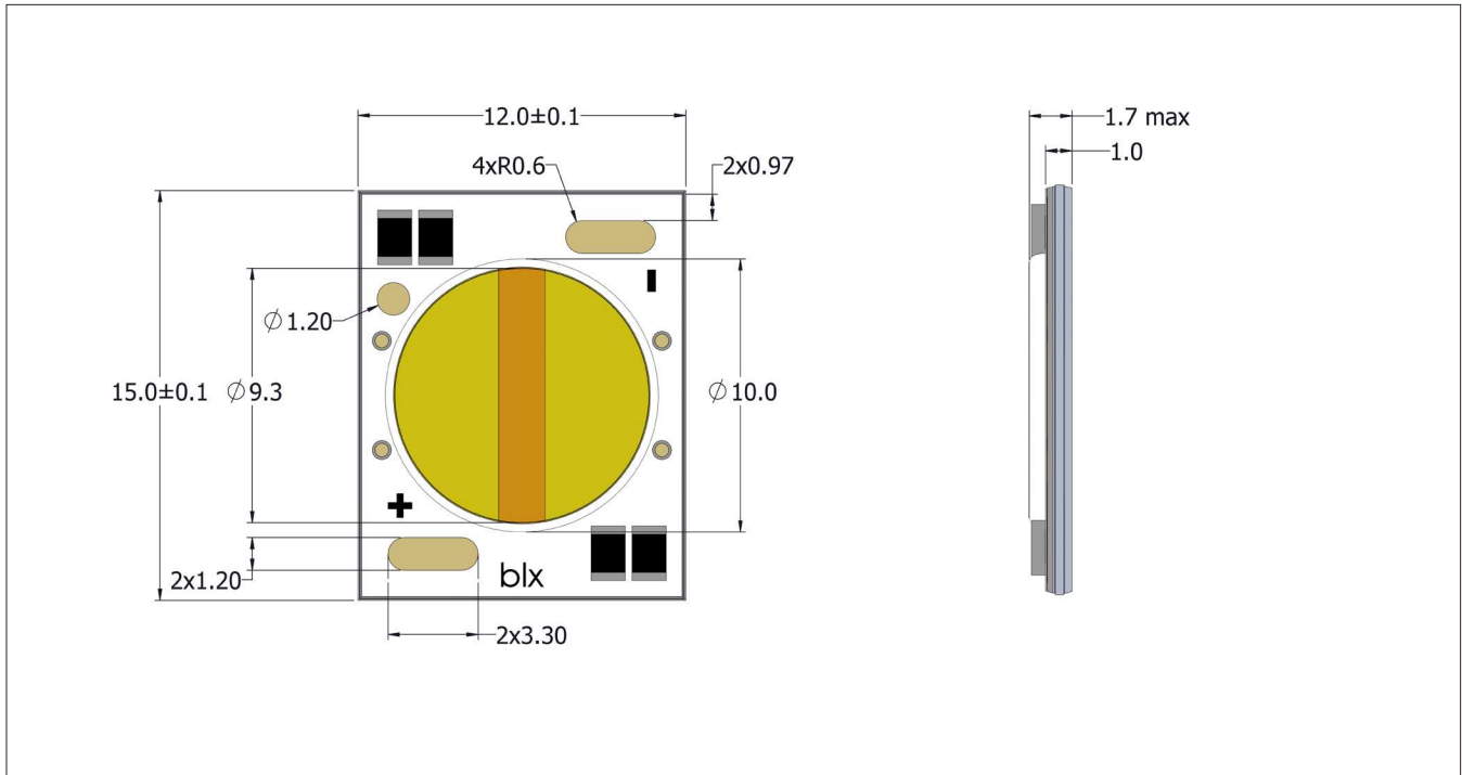
Figure 18: Drawings for Vesta Dim-To-Warm gmm Array
