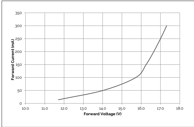
Figure 1: 4W Forward Voltage vs. Forward Current, T_c=25^\circ\text{C}
