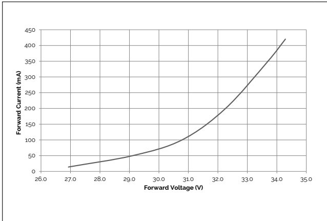
Figure 3: 12W Forward Voltage vs. Forward Current, T_c=25^\circ\text{C}
