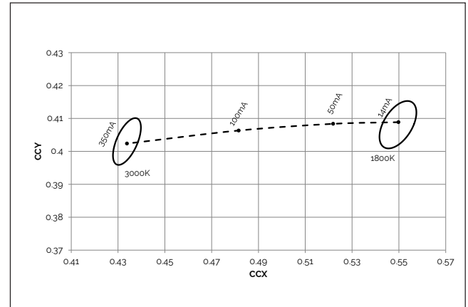
Figure 12: Color shift vs. Forward Current 3000K - 1800K
