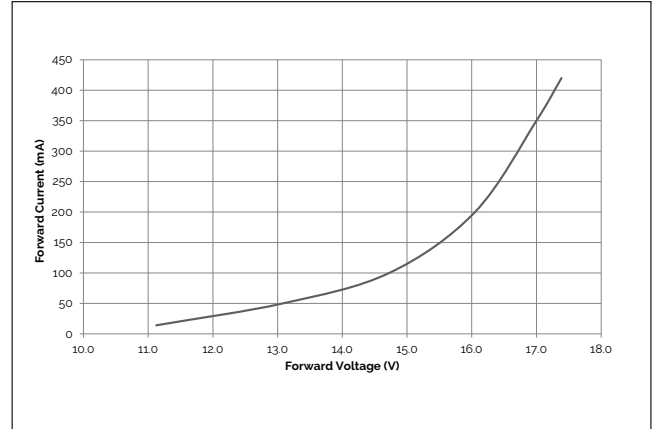
Figure 2: 6W Forward Voltage vs. Forward Current, T_c=25^\circ\text{C}
