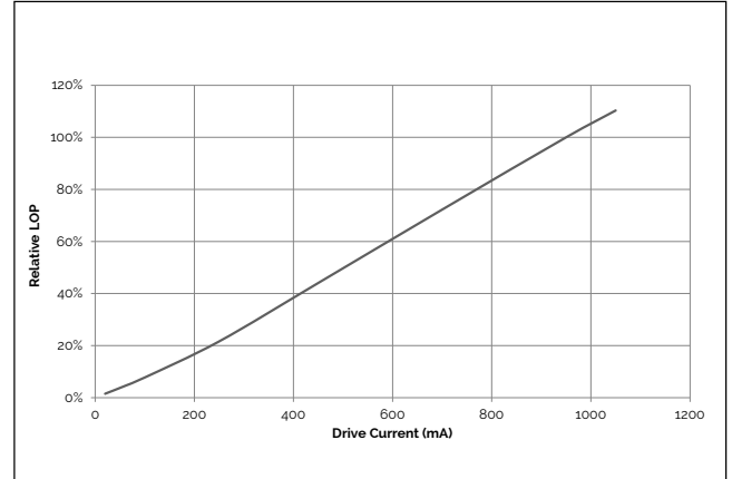
Figure 2: Relative LOP vs. Drive Current, T_c=25^\circ\text{C}
