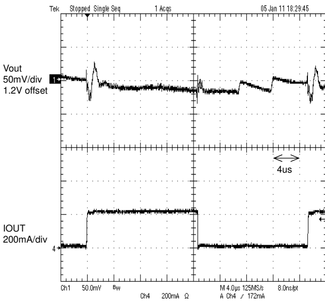
Figure 23. Load transient response 5mA to 200mA tr=tr=100ns , MODE : Low
