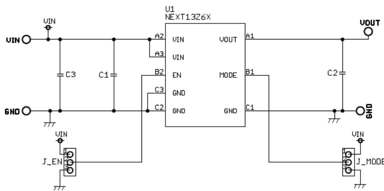
Figure 40. PCB Circuit
