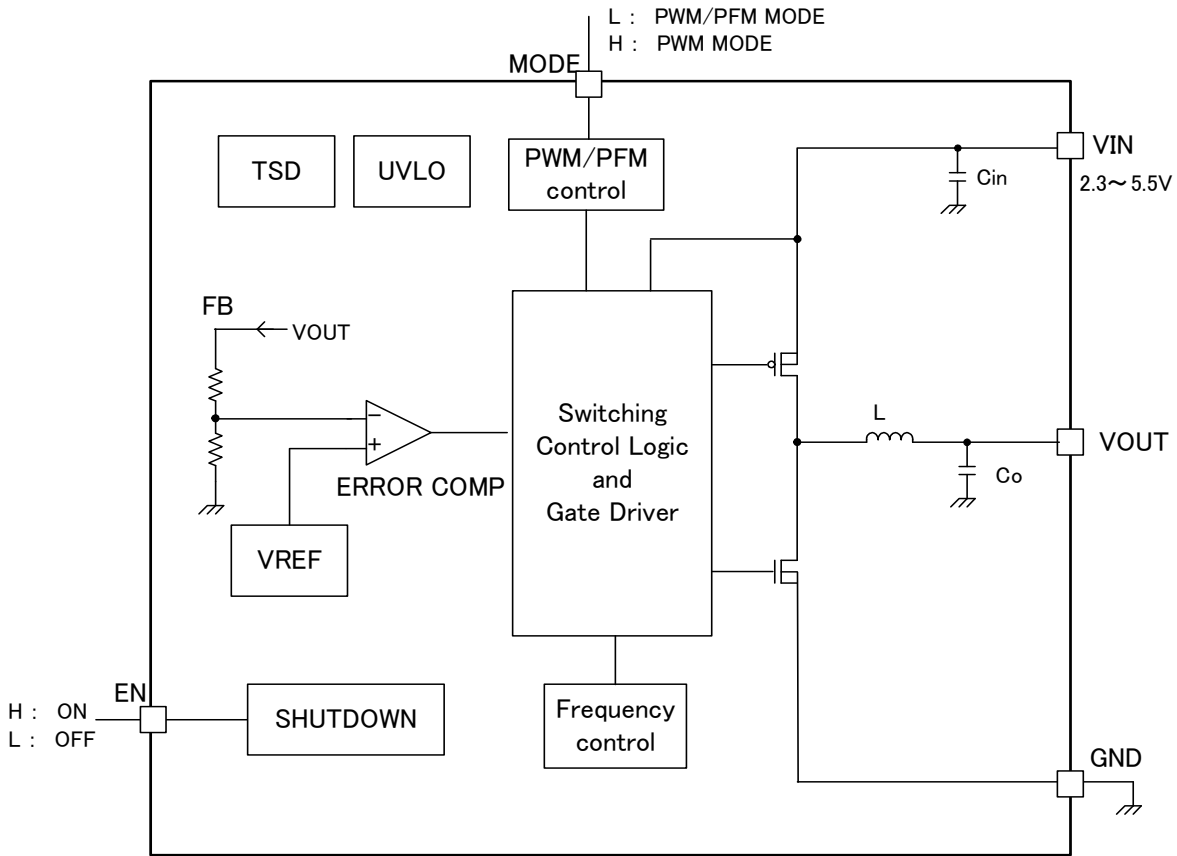
Figure 3. Block Diagram(s)
