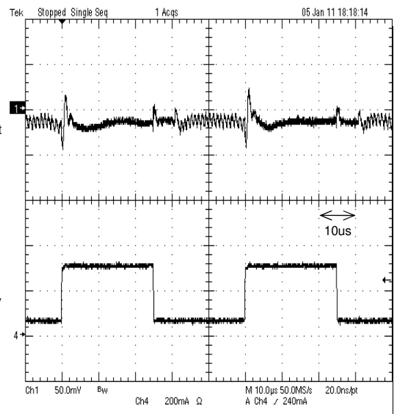
Figure 24. Load transient response 50mA to 350mA tr=tr=100ns , MODE : Low
