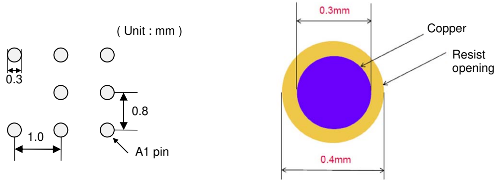
Figure 37. Recommended Land Pattern (TOP VIEW)
