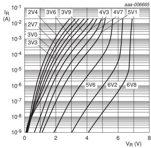
BZX384-B/C2V4 to BZX384-B/C6V8 T_{amb} = 25\text{ °C}
