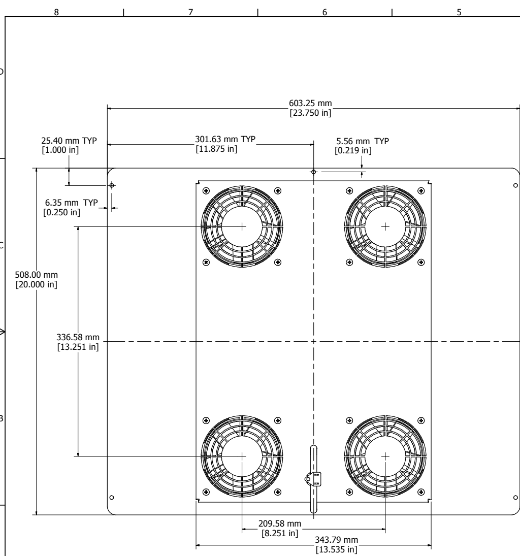
ASSEMBLY - VIEW FROM BOTTOM
