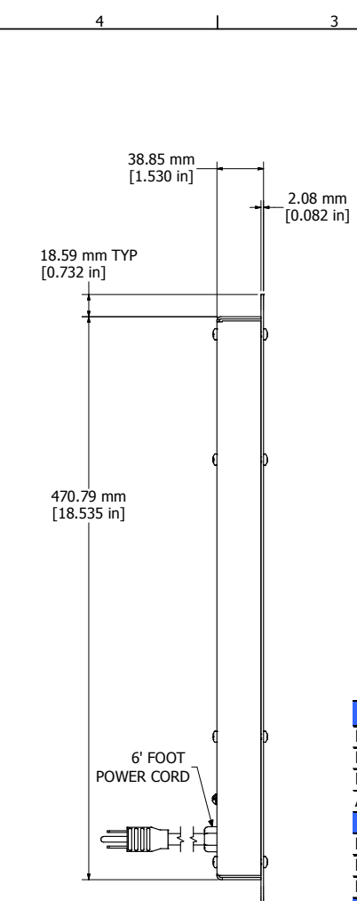
ASSEMBLY - VIEW FROM SIDE
