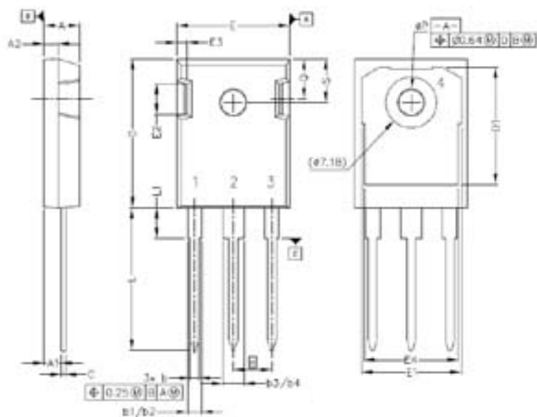
Package TO-247-3
