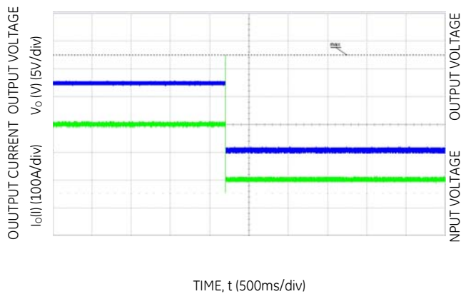
Figure 11. Overload: output short circuit performance, the unit is in latch_OFF mode. , V IN = -48V DC .
