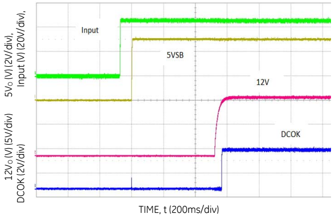
Figure 2. Input start up (Vin: -48V DC , full load).
