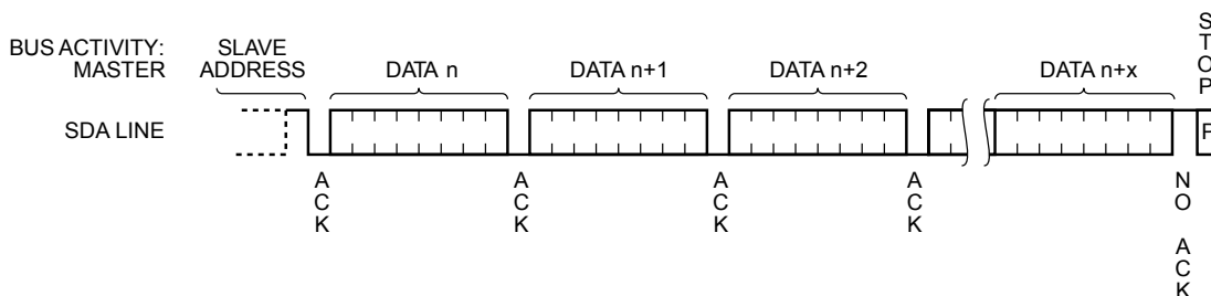
Figure 11. Sequential Read Timing
