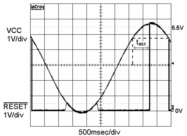
Transient Response
