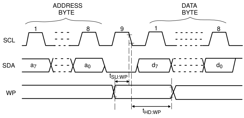
Figure 9. WP Timing
