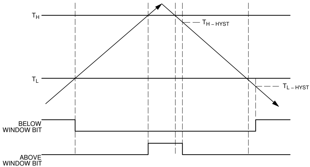
Figure 10. Hysteresis Detail
