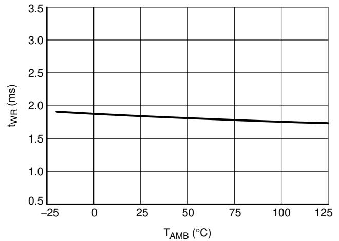
Figure 13. EEPROM Write Time (Rev. C)
