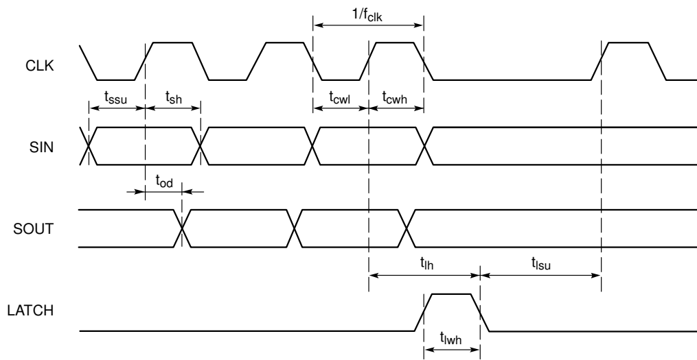
Figure 3. Serial Input Timing Diagram
