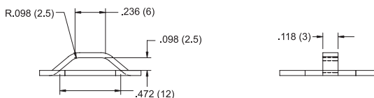
Recommended Mounting Slot
