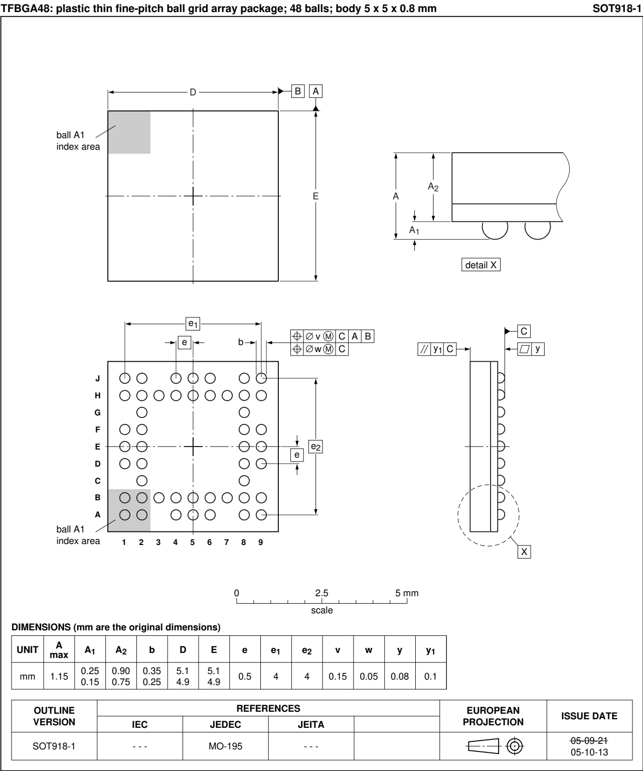
Fig 4. Package outline TFBGA48 (SOT918-1)
