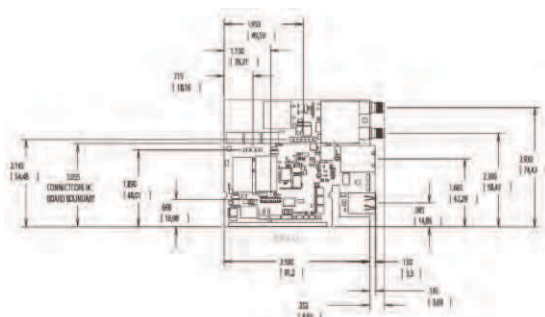
ConnectCore 9C/Wi-9C Top View
