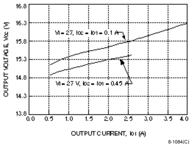
Figure 8. CC025ACL-M Typical Cross Regulation with Respect to I_{ol}
