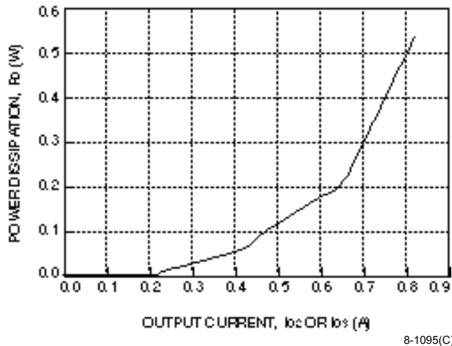
Figure 27. CC025ACL-M Losses Associated with ±15 V Output, Ps2/Ps3
