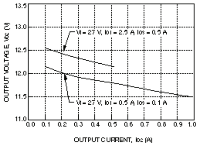
Figure 5. CC025ABK-M Typical Load Regulation
