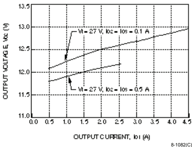
Figure 6. CC025ABK-M Typical Cross Regulation with Respect to I_{ol}
