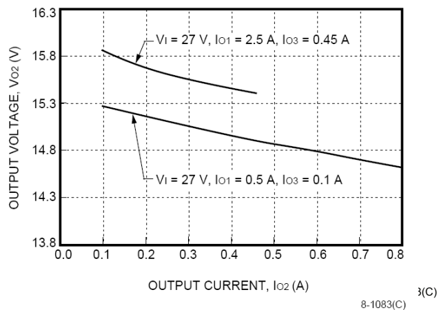
Figure 7. CC025ACL-M Typical Load Regulation
