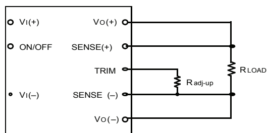
Figure 18. Circuit Configuration to Increase Output Voltage
