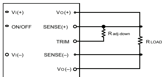
Figure 19. Circuit Configuration to Decrease Output Voltage
