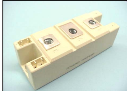
CD63_15B Dual SCR Isolated POW-R-BLOK™ Module 150 Amperes / Up to 1800 Volts
