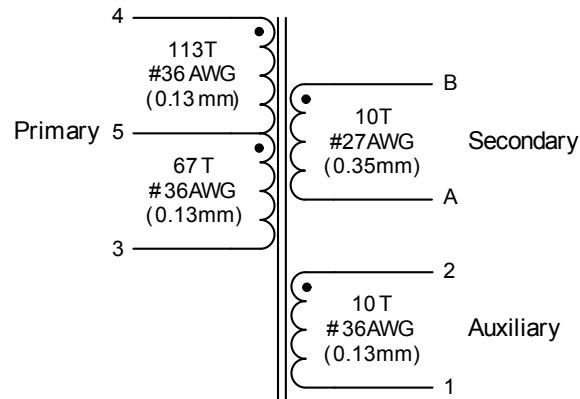
Figure 8. Flyback Transformer Schematic
