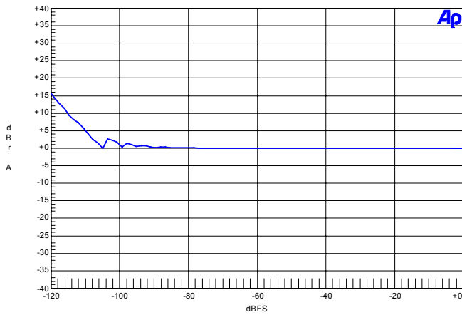
Figure 22. 96 kHz, Fade-to-Noise Linearity
