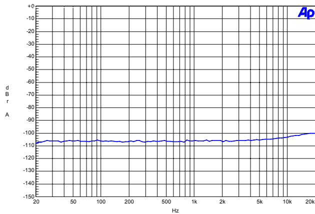
Figure 24. 96 kHz, Crosstalk
