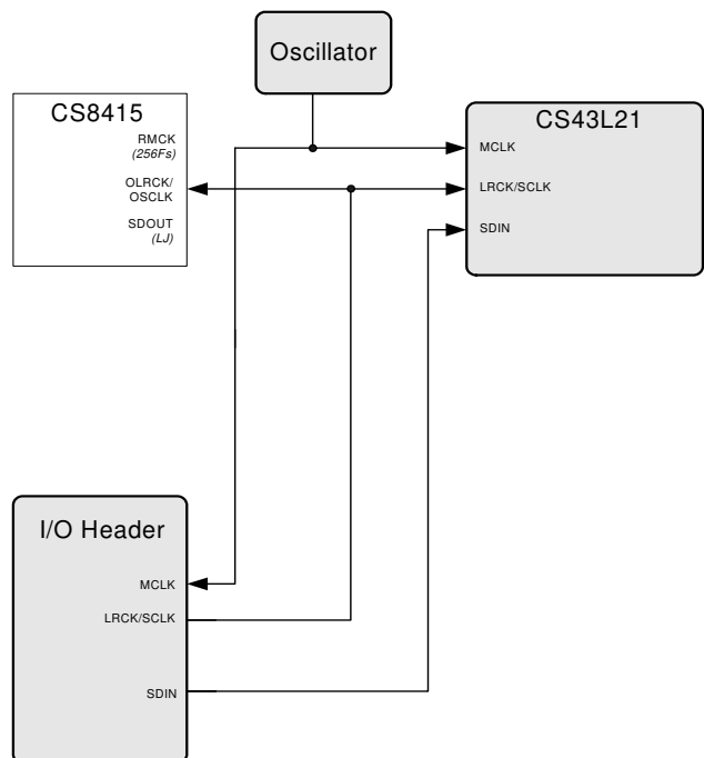
Figure 7. Routing 4
