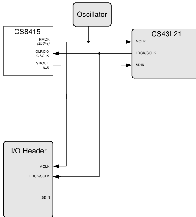
Figure 8. Routing 5
