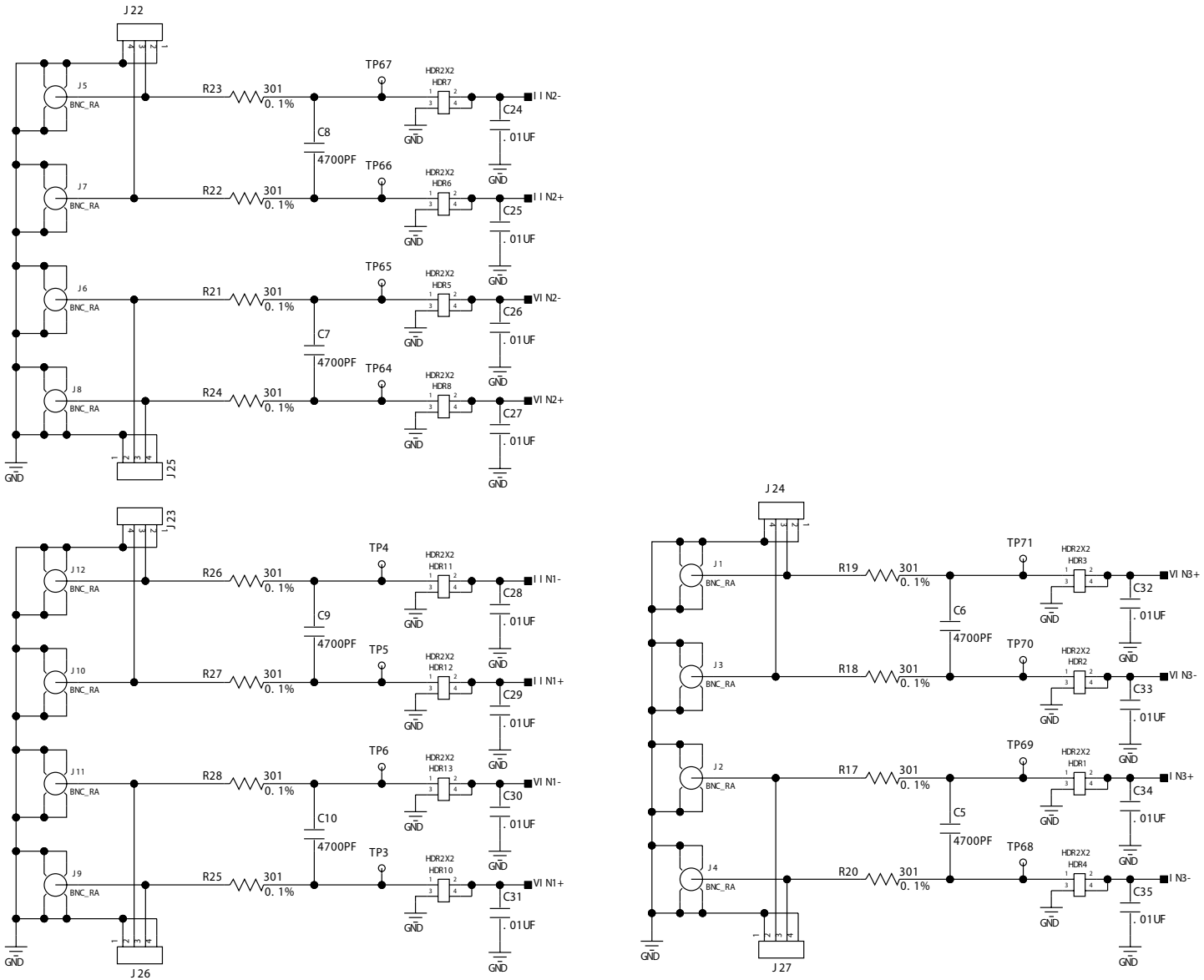
Figure 2. Analog Inputs
