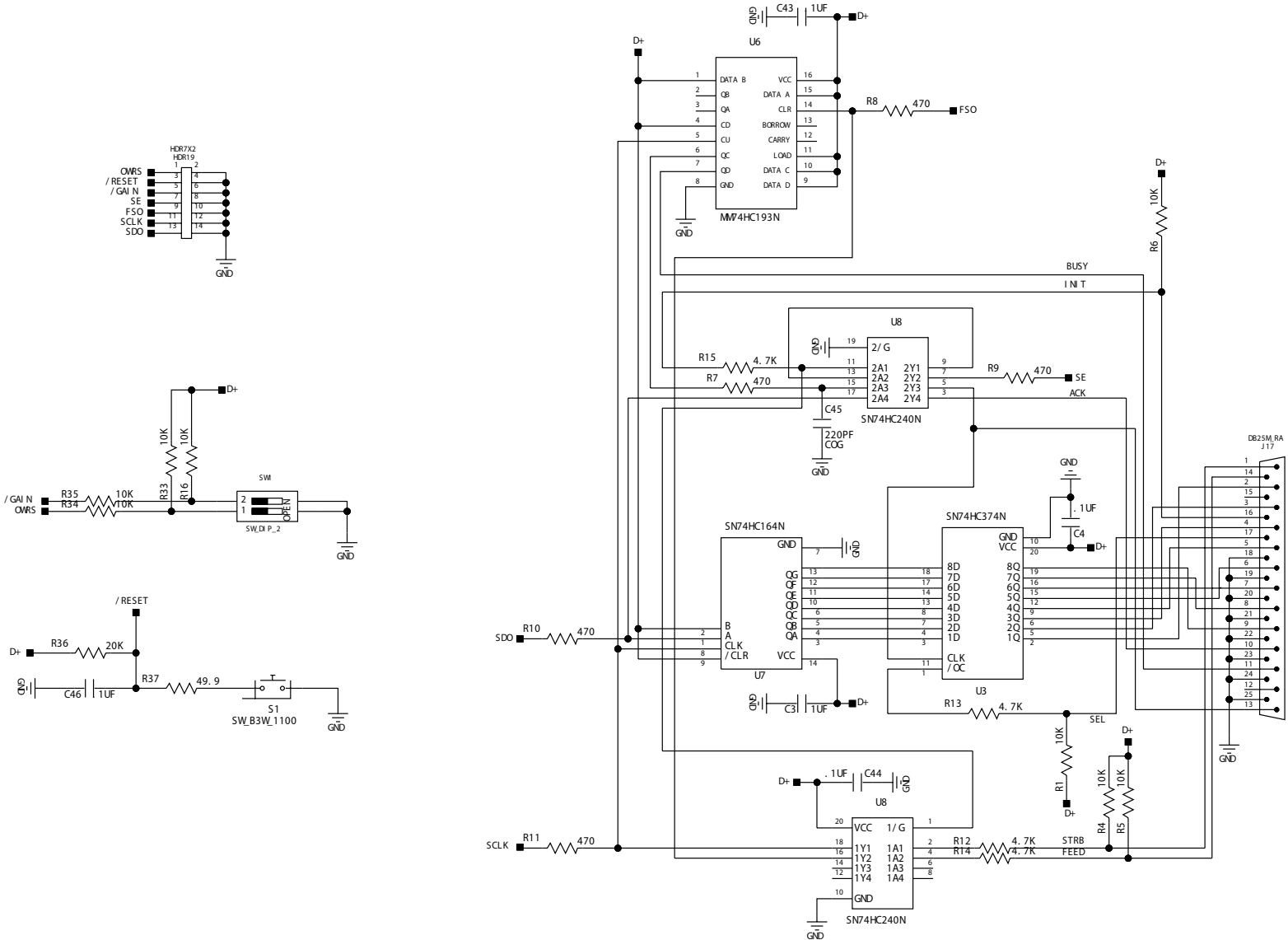
Figure 3. Digital Circuitry
