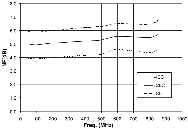
Noise Figure vs. Frequency Over Temperature
