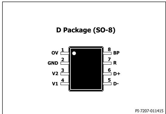
Figure 4. Pin Configuration.
