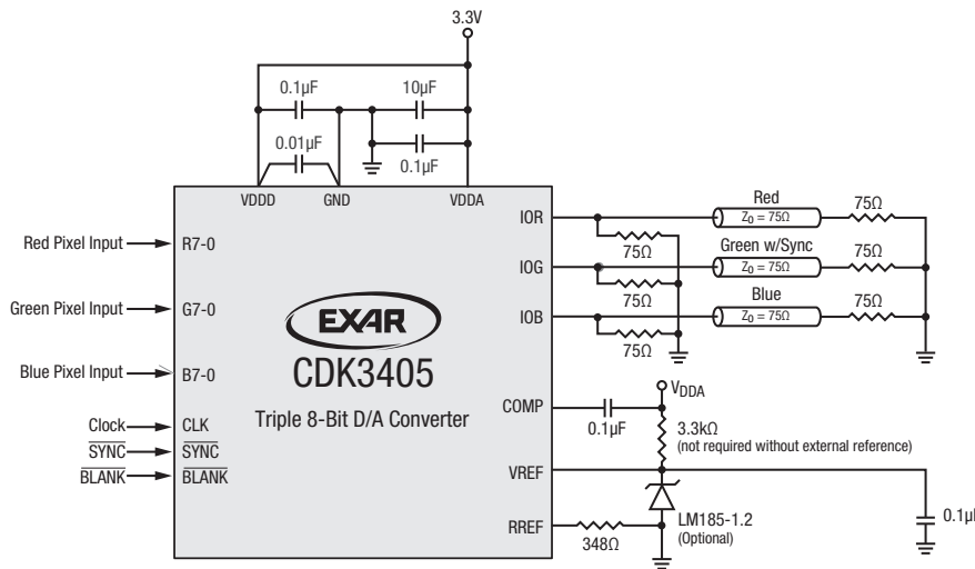
Typical Interface Circuit Diagram
