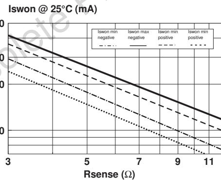
Fig. 30 : Variation of switching-on current versus R_{SENSE} at 25^\circ C .
