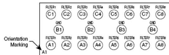
CM1450-08CS/CP 20-Bump CSP Package
