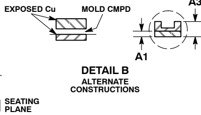
DETAIL A ALTERNATE CONSTRUCTIONS
